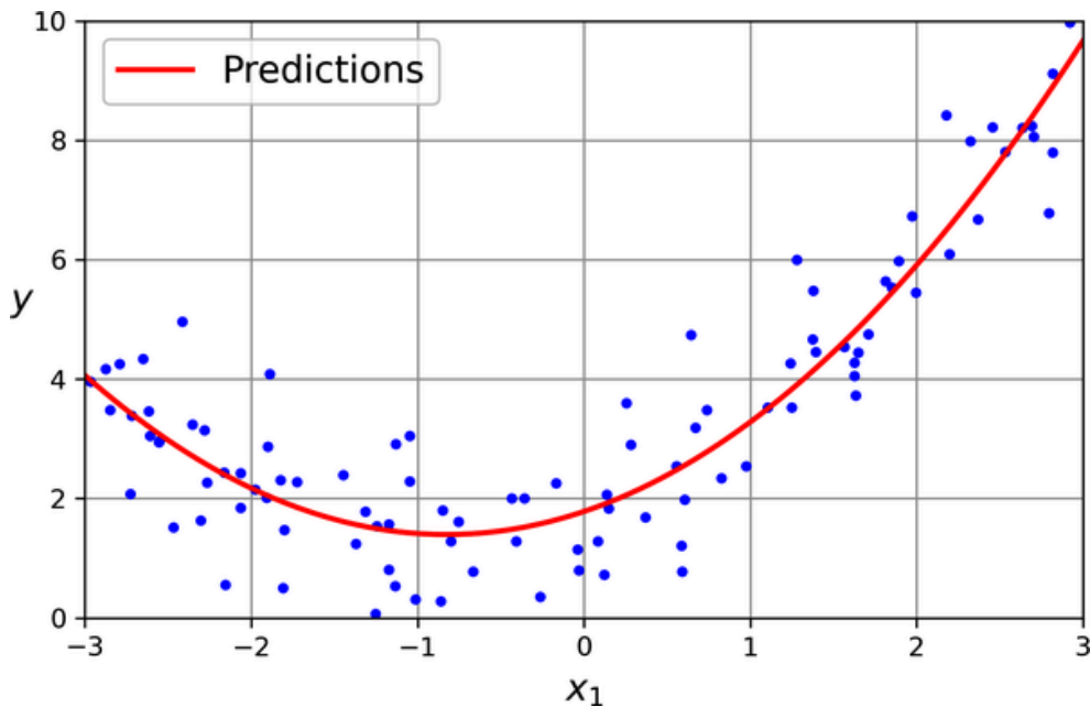
Figure 4-13. Polynomial regression model predictions
