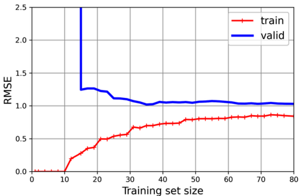
Figure 4-16. Learning curves for the 10th-degree polynomial model
