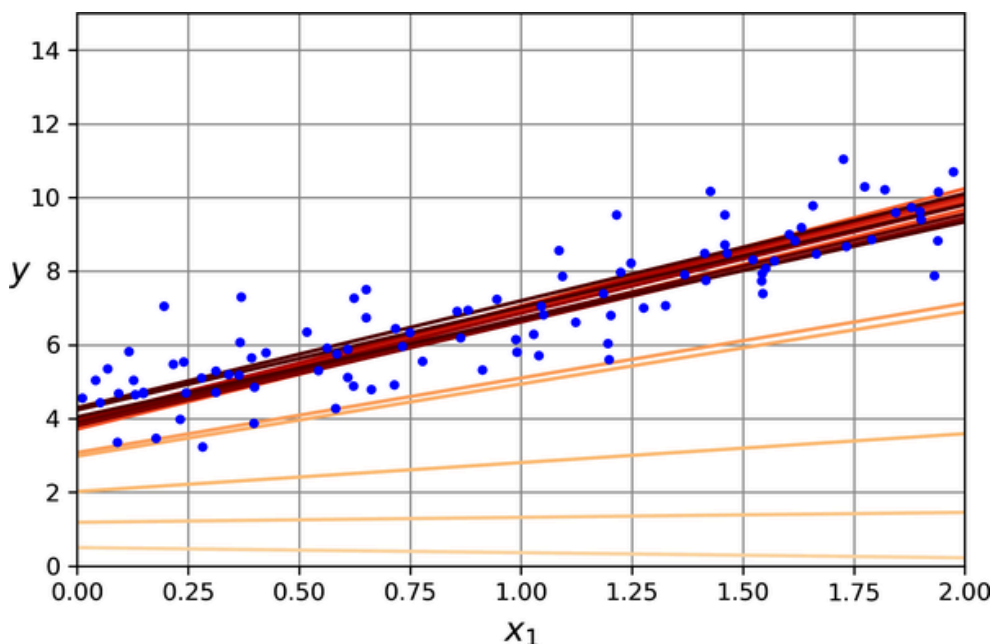
Figure 4-10. The first 20 steps of stochastic gradient descent
