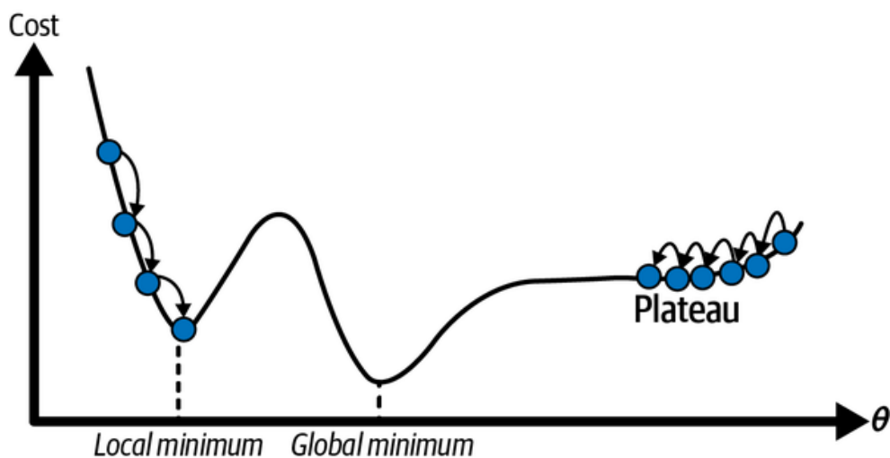
Figure 4-6. Gradient descent pitfalls
