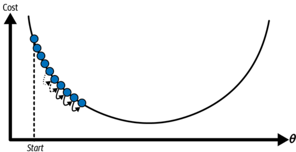
Figure 4-4. Learning rate too small
