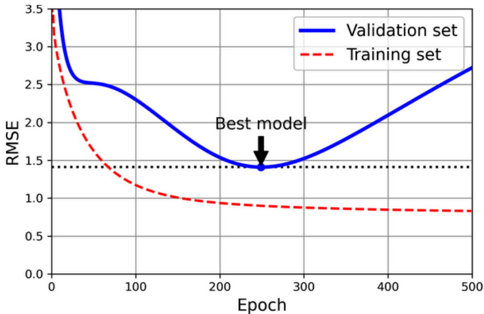
Figure 4-20. Early stopping regularization
