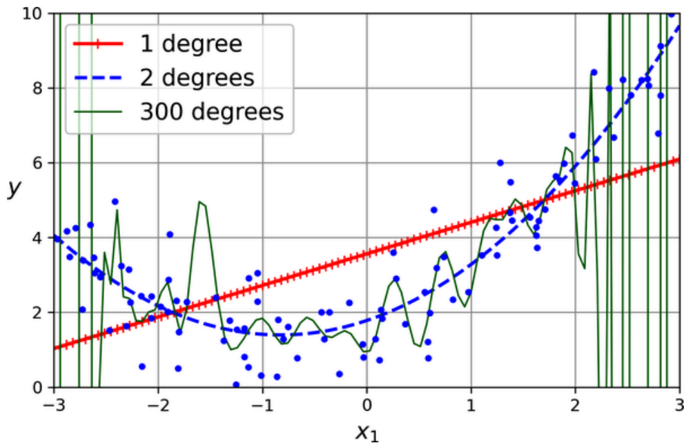
Figure 4-14. High-degree polynomial regression
