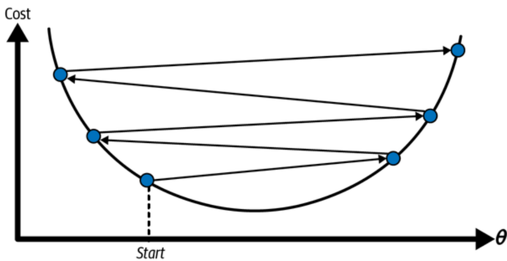
Figure 4-5. Learning rate too high
